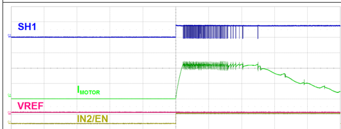
Figure 56. Current Profile on Motor Startup With Regulation
