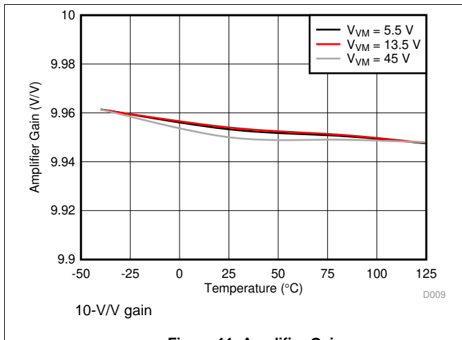
Figure 11. Amplifier Gain
