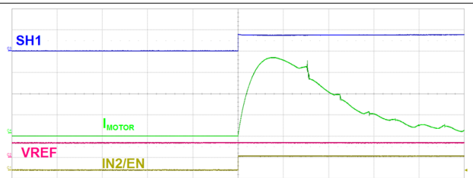
Figure 57. Current Profile on Motor Startup Without Regulation
