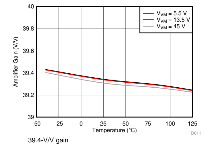
Figure 13. Amplifier Gain
