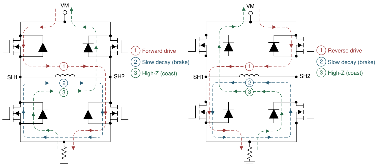
Figure 31. Bridge Control
