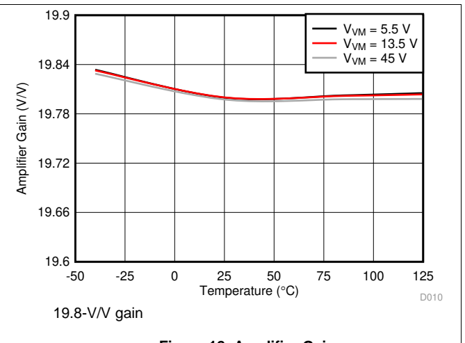
Figure 12. Amplifier Gain
