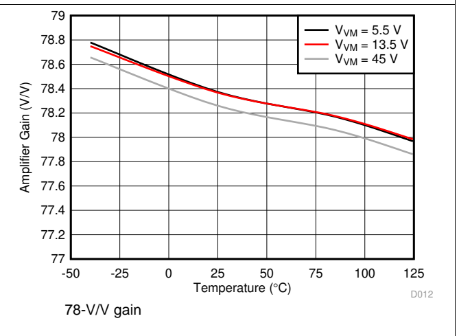
Figure 14. Amplifier Gain
